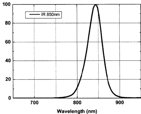
Wavelength Spectrum, Ta=25°C Typical Polar Radiation Pattern
